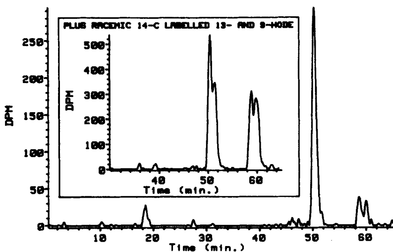
Fig. 7. Representative straight-phase chiral HPLC radiochromatograms of the methyl esters of the radiolabeled 13- ^{14}\text{C} ]HODE and 9- ^{14}\text{C} ]HODE produced in the incubation of ^{14}\text{C} ]linoleic acid with hair roots epilated from the scalp of a normal male. The outer chromatogram is that of the material in the peak at 20.5 min (Fig. 2, upper chromatogram) which was then subjected to the chiral-phase chromatography shown here. The methyl ester of 13-HODE elutes prior to that of 9-HODE and the S -stereoisomer of each compound is the first to elute under these chromatographic conditions. The chromatogram shown in the inset is that of an equal aliquot of the same material to which racemic 13- ^{14}\text{C} ]HODE and 9- ^{14}\text{C} ]HODE methyl ester standards had been added. The mixing experiment demonstrates that the principal product of the incubation of linoleic acid with hair roots is 13( S )-HODE, with racemic 9-HODE constituting a minor product.
