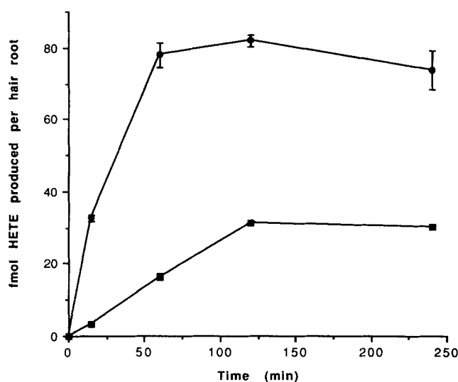
Fig. 2. Time course for the production of 15- ^3\text{H} HETE (solid squares) and 12- ^3\text{H} HETE (solid circles) from [ ^3\text{H} ]arachidonic acid by anagen hair roots. Twenty-six beard anagen hair roots, suspended in 1 ml medium, were incubated at 37°C in the presence of 4 \mu\text{Ci} [ ^3\text{H} ]arachidonic acid. Triplicate aliquots of 50 \mu\text{l} each were taken at the time points shown and the amounts of 15- ^3\text{H} HETE and 12- ^3\text{H} HETE were measured in each using reversed-phase HPLC with radioactive monitoring of the eluate. Standard error bars are drawn for each time point. The results shown here are representative of the three time course experiments that were performed.
