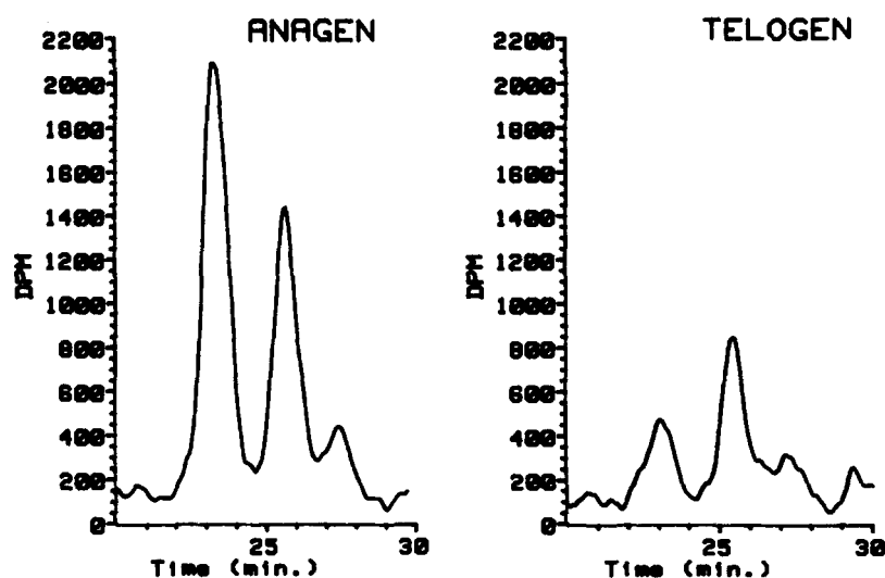
Fig. 8. Reversed-phase HPLC radiochromatograms of the radiolabeled products of the incubation of [ ^3\text{H} ]arachidonic acid with anagen (left panel) and telogen (right panel) hair roots from the scalp of a normal male. The production of 15- and 12-HETE was consistently higher in the anagen hair roots. However, the difference in the relative production of the two HETEs by the anagen and telogen hair roots, observed in this experiment, was not a consistent finding.
