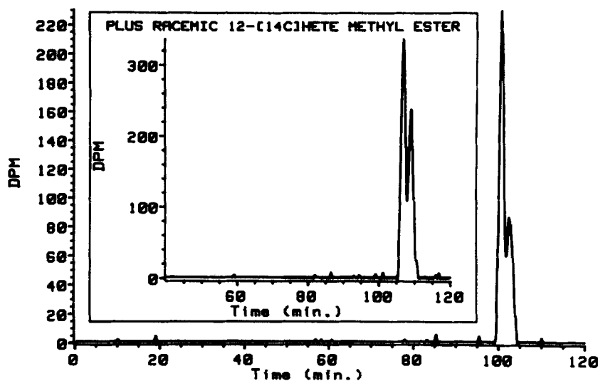
Fig. 6. Representative straight-phase chiral HPLC radiochromatograms of the methyl ester of the radiolabeled 12- ^{14}\text{C} ]HETE produced in the incubation of ^{14}\text{C} ]arachidonic acid with hair roots epilated from the beard of a normal male. The outer chromatogram is that of material eluting at 25 min on reversed-phase HPLC (as in Fig. 1) that was collected, methylated, and re-chromatographed on straight-phase columns prior to the chiral-phase chromatography shown here. The chromatogram shown in the inset is that of an equal aliquot of the same material to which racemic 12- ^{14}\text{C} ]HETE methyl ester standard had been added. The S/R ratio of the experimentally produced material was 2.2 and this ratio decreased, as expected, following the addition of racemic 12- ^{14}\text{C} ]HETE methyl ester standard.
